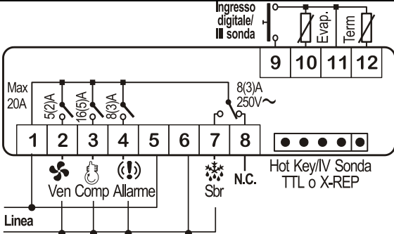
16.1 VERDICHTER-RELAIS 8A OD. 16A - 120VAC OD. 230 VAC
